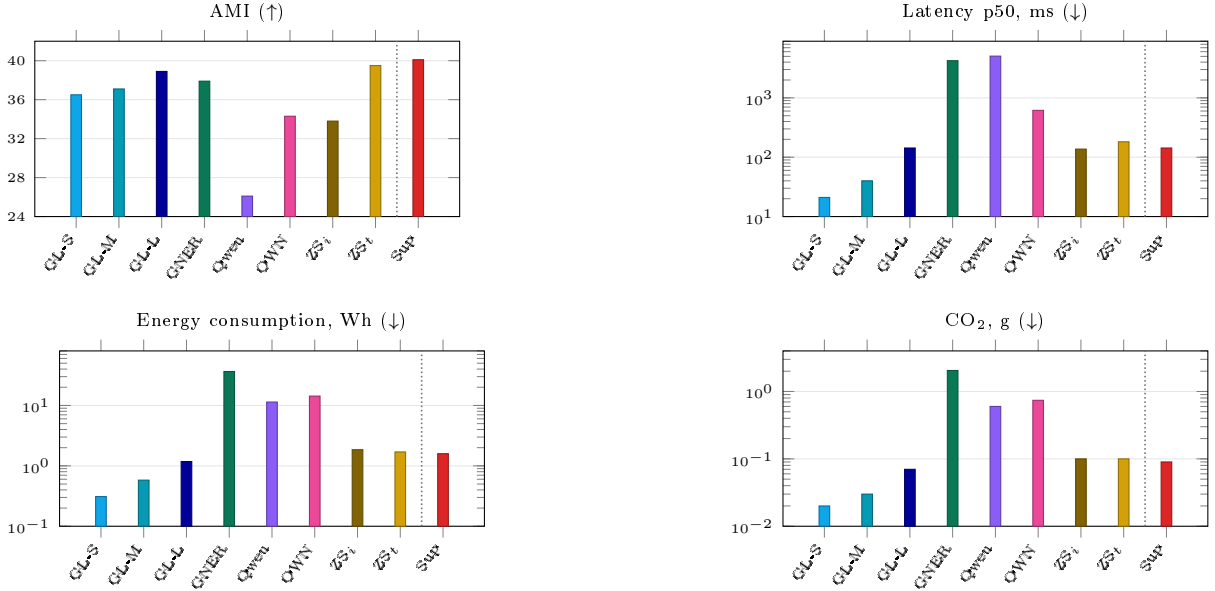
Fig. 6 Per-model means on the four axes (13-set averages, Table 8). The light dotted line separates the zero-shot systems (left) from the supervised OPENER-Sup (right). Latency, energy and CO 2 use a log scale. Labels: GL-S/M/L = GLiNER sizes, OWN = OWNER, ZS i = OPENER-ZS ind , ZS t = OPENER-ZS trans , Sup = OPENER-Sup
