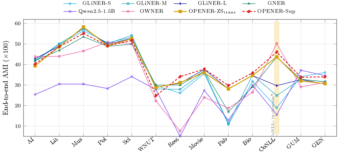
Fig. 3 End-to-end AMI per dataset (Table 5, OPENER curves show the three-seed means). Zero-shot systems are drawn solid. OPENER-Sup is the dashed red line. a CoNLL-2003 (shaded) is in-domain for OWNER and OPENER. b Qwen is evaluated on a 150-sentence subsample per set
