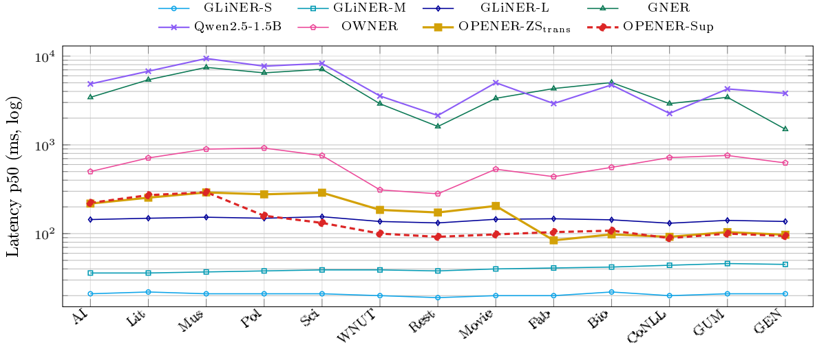
Fig. 4 Per-sentence inference latency (p50, ms, log scale) per dataset (Table 6). Same systems and styling as Figure 3. OPENER-Sup is the dashed red line. The OPENER variants track GLiNER-L, while GNER and the Qwen LLM are one to two orders of magnitude slower
