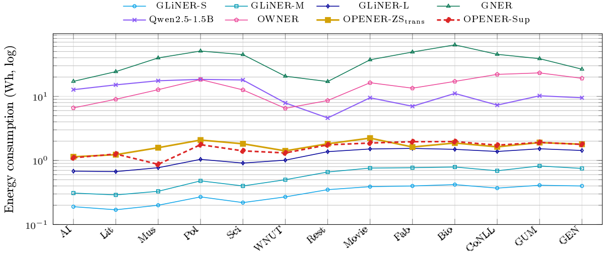
Fig. 5 Per-run energy consumption (Wh, log scale) per dataset (Table 7). Same systems and styling as Figure 3. The OPENER variants sit an order of magnitude below OWNER and the generative GNER/Qwen baselines
