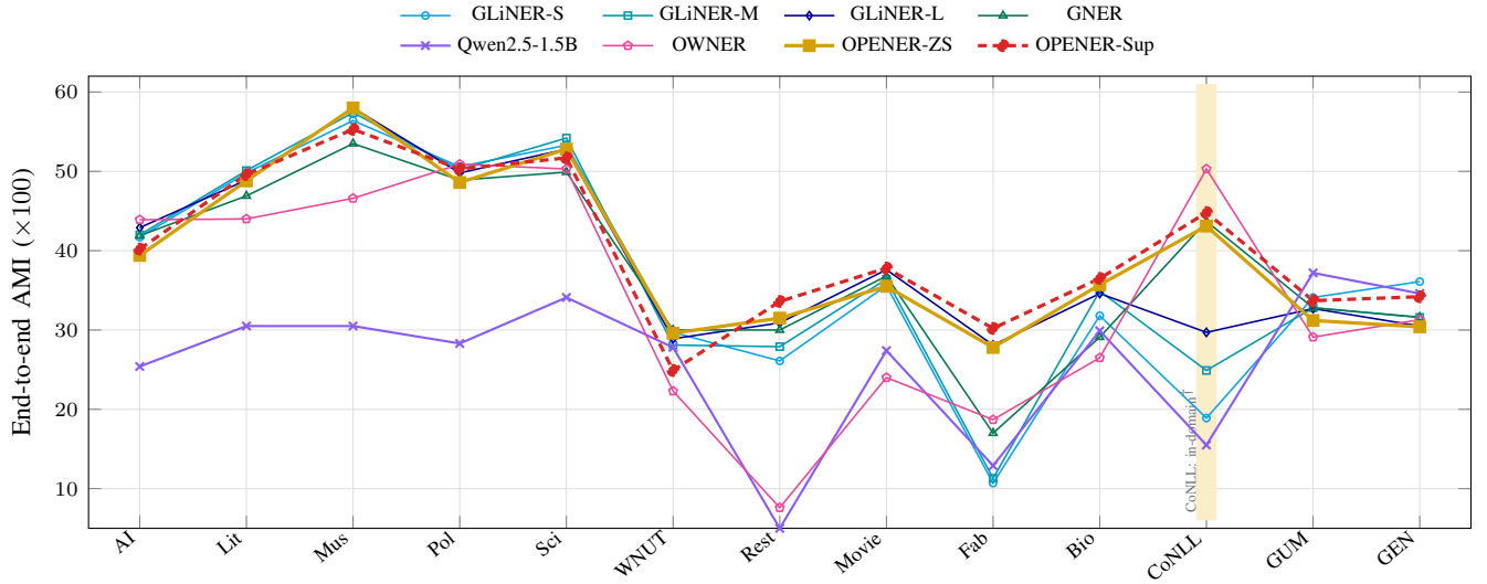
Fig. 2. End-to-end AMI per dataset (Table III). Zero-shot systems are drawn solid; OPENER-Sup (the supervised upper bound) is the dashed red line. \dagger CoNLL-2003 (shaded) is in-domain for OWNER and OPENER; \ddagger Qwen is evaluated on a 150-sentence subsample per set.
