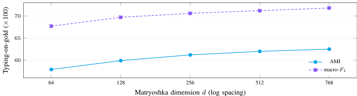
Fig. 7. Typing-on-gold quality vs the Matryoshka truncation dimension d (Table IX, dimension axis; released seed, 13-set means, log-spaced d ). Both AMI and macro- F_1 degrade smoothly with diminishing returns and flatten above d=256 , showing that truncation is a graceful cost/quality knob and that the Matryoshka structure survives the contrastive fine-tuning.
