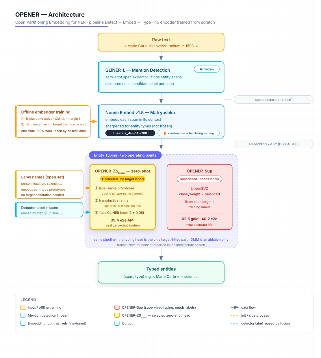
Fig. 1. The OPENER pipeline (Detect → Embed → Type): a frozen GLiNER detector proposes spans, a Matryoshka embedder (Nomic, contrastively fine-tuned) maps each span in context to a vector, and a typing head assigns a type. The typing head (the only target-fitted component) has two operating points: the zero-shot OPENER-ZS trans (★, selected) and OPENER-Sup ( supervised , the upper bound). All upstream components are ready-to-use.
