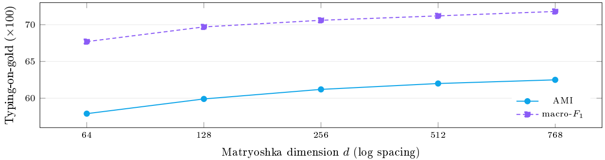
Figure 7: Typing-on-gold quality vs the Matryoshka truncation dimension d . Both AMI and macro- F_1 degrade smoothly, with diminishing returns rather than a cliff, and flatten above d=256 . Truncation is therefore a graceful cost/quality knob, and the Matryoshka structure survives the contrastive fine-tuning. Data from Table 9 (dimension axis, released seed, 13-set means, log-spaced d ).
