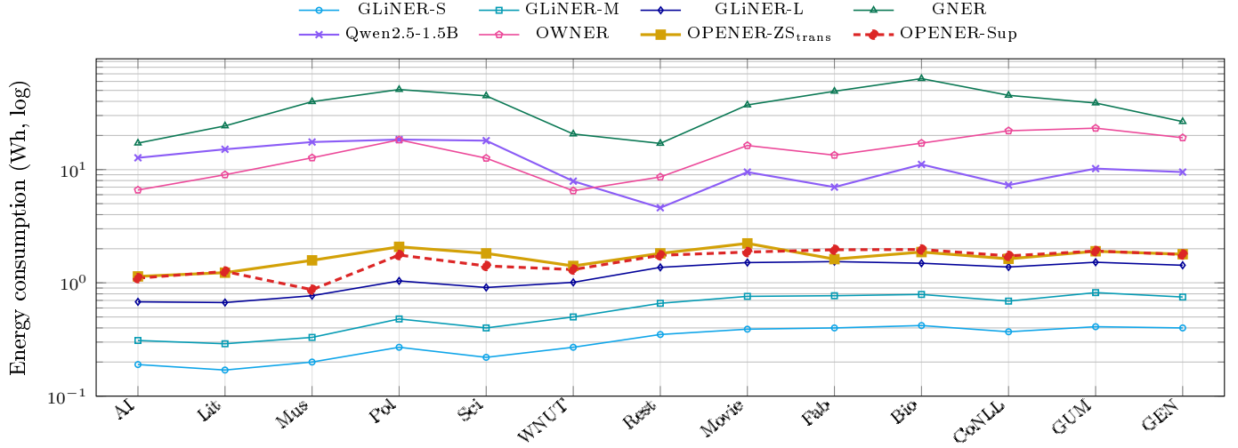
Figure 4: Per-run energy consumption (Wh, log scale) per dataset (Table 7). Same systems and styling as Figure 2. The OPENER variants sit an order of magnitude below OWNER and the generative GNER/Qwen baselines.
