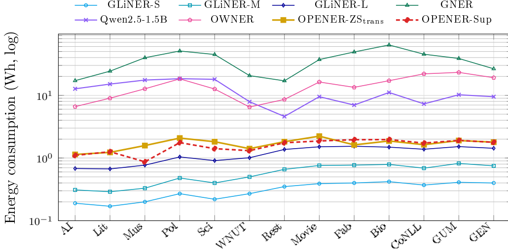
Figure 4: Per-run energy consumption (Wh, log scale) per dataset (Table 7). Same systems and styling as Figure 2. The OPENER variants sit an order of magnitude below OWNER and the generative GNER/Qwen baselines.
