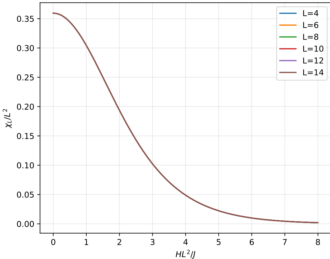
Scaling de Binder-Landau, T = 2.1
