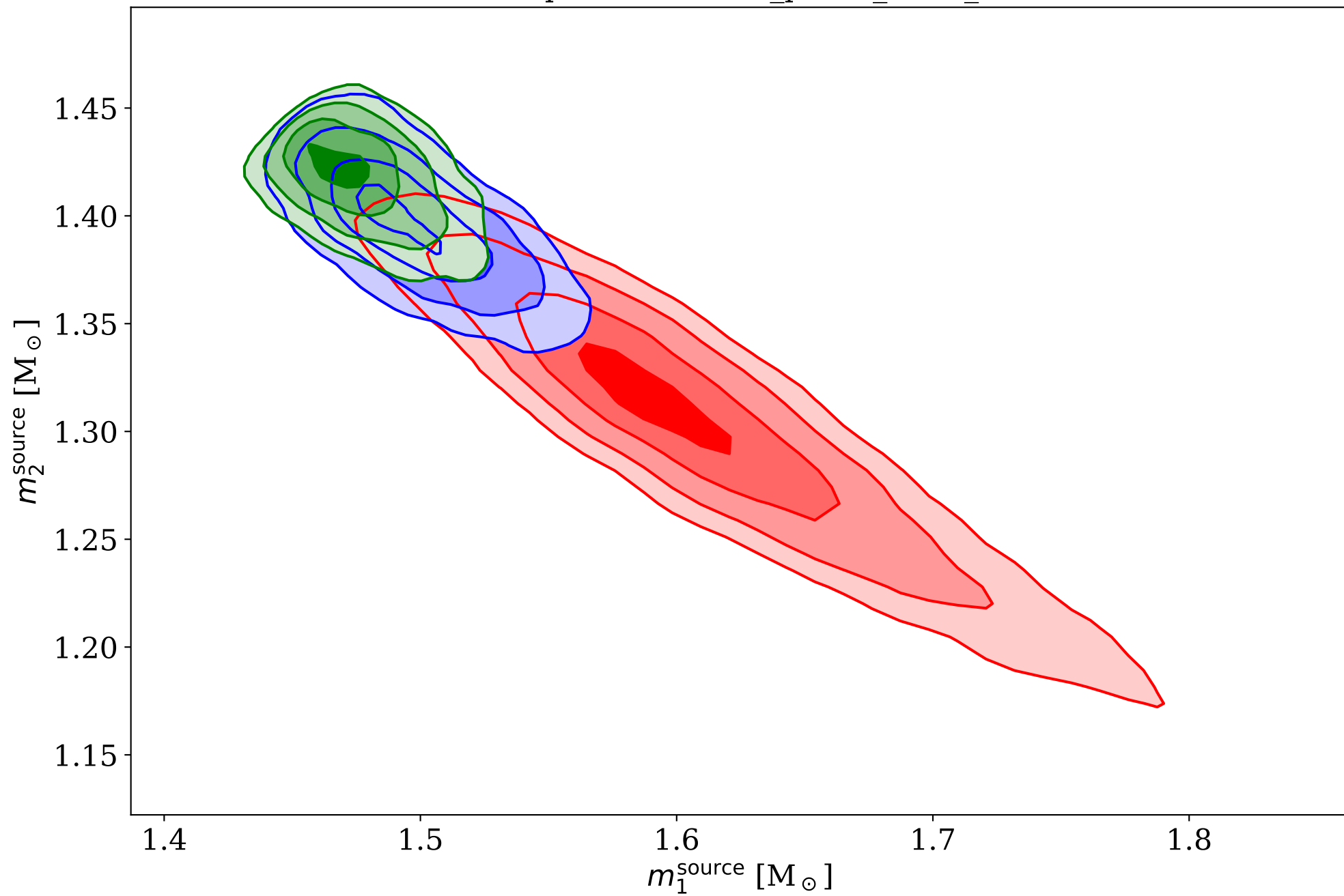
Mass comparison: neural_priors_radio_chiEFT
