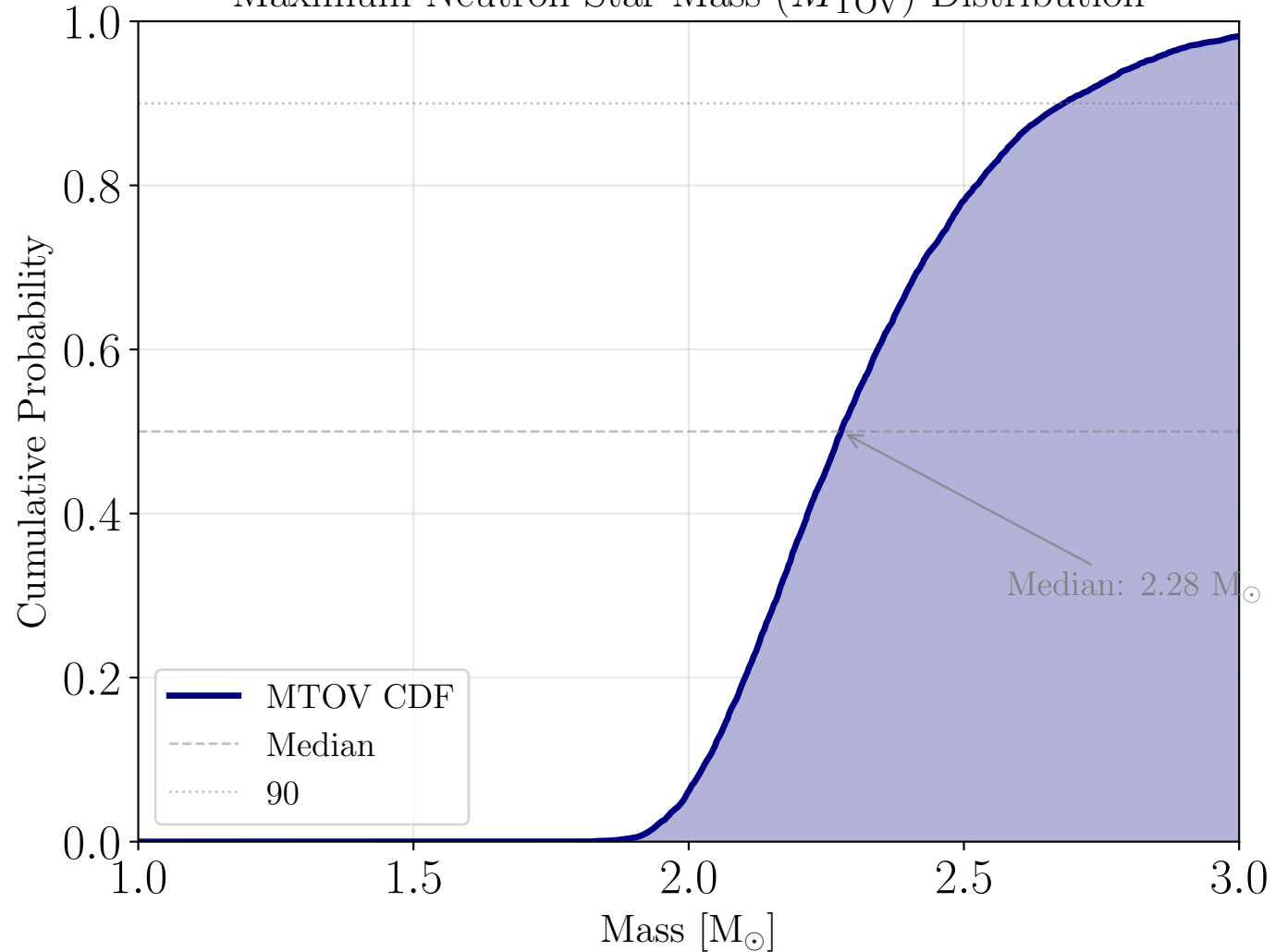
Maximum Neutron Star Mass ( M_{\text{TOV}} ) Distribution
