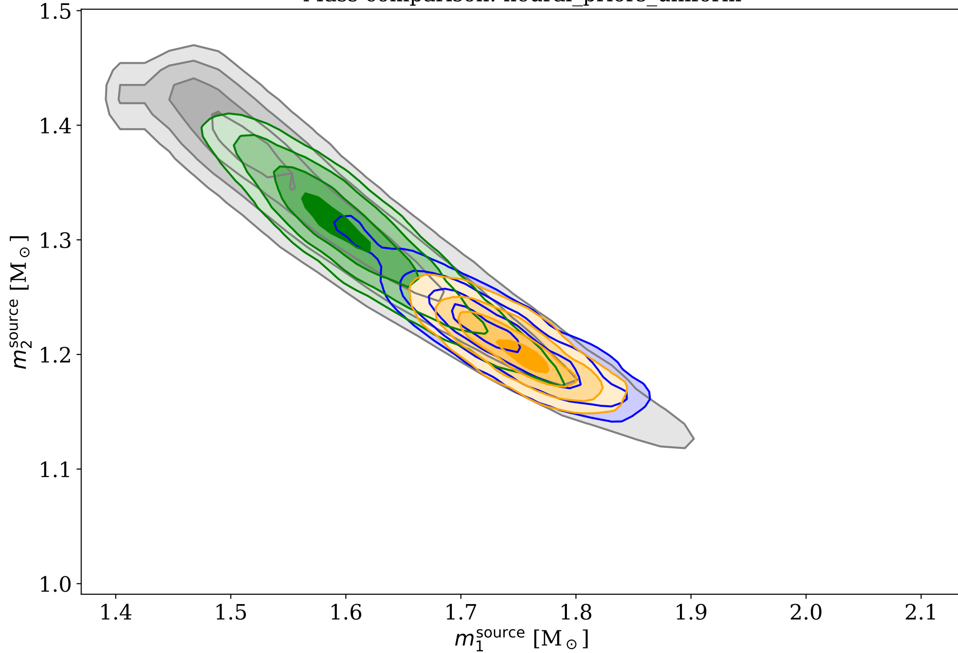
Mass comparison: neural_priors_uniform
