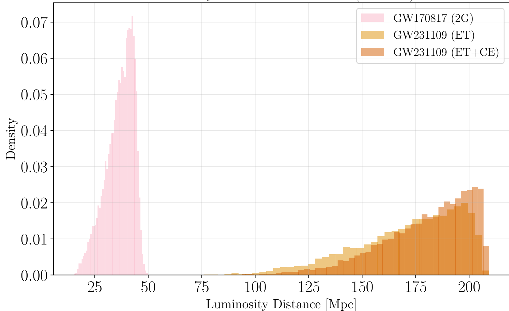
Luminosity Distance Distributions (DEBUG)
