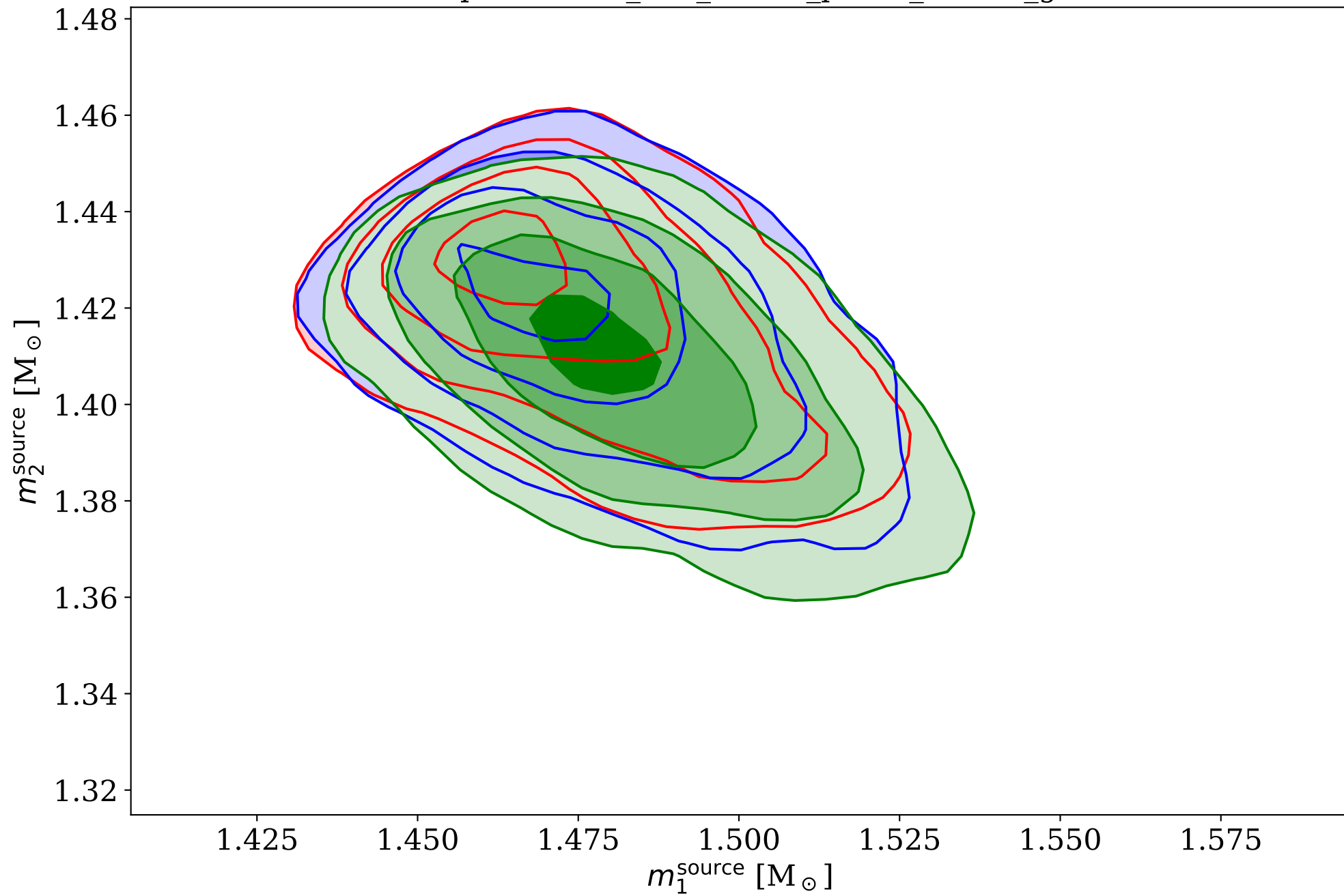
Mass comparison: no_test_neural_priors_double_gaussian
