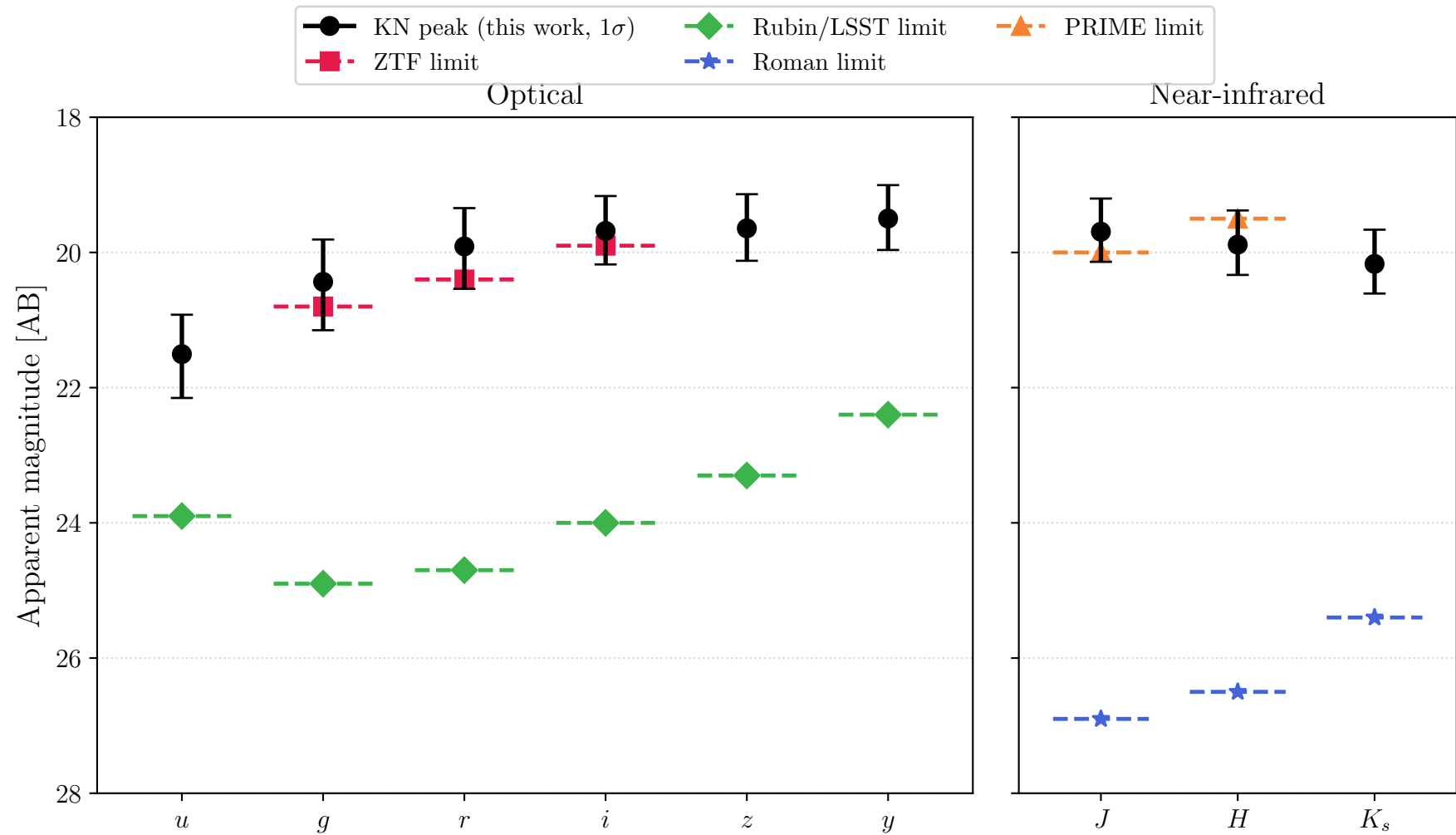
GW231109 kilonova peak magnitude vs. instrument limits
