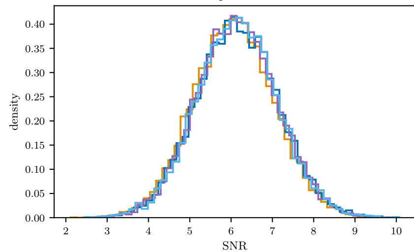
H1 matched filter snr
