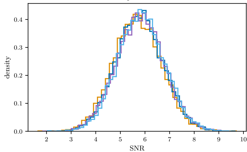
L1 matched filter snr
