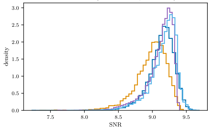
network SNR (matched-filter, \sqrt{H^2 + L^2} )
