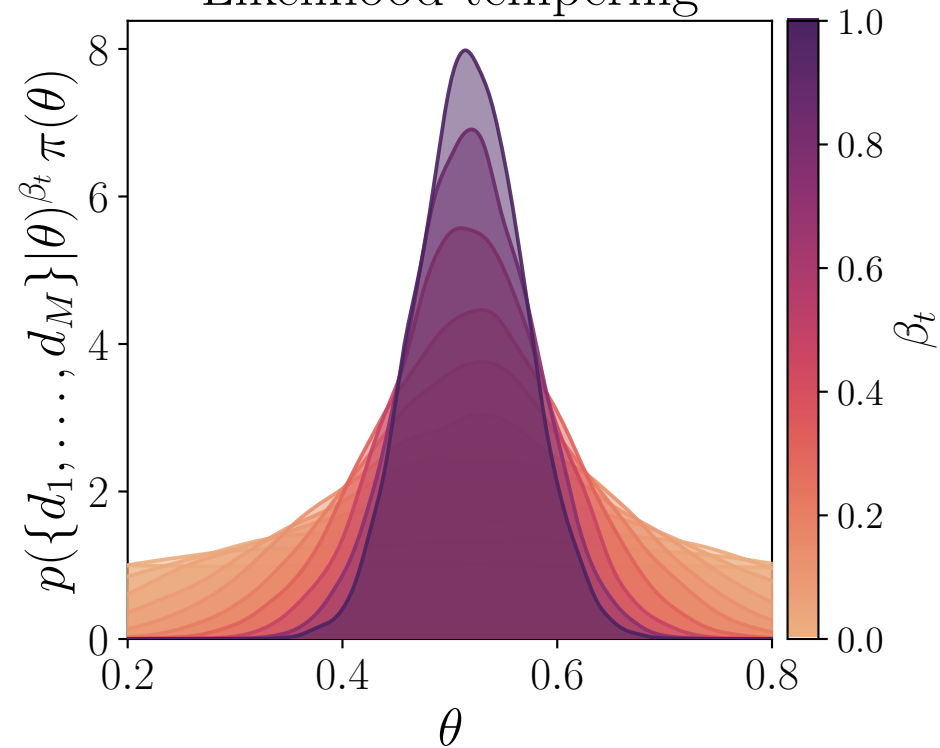
Likelihood tempering
