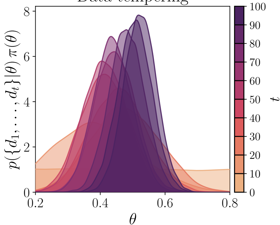
Data tempering
