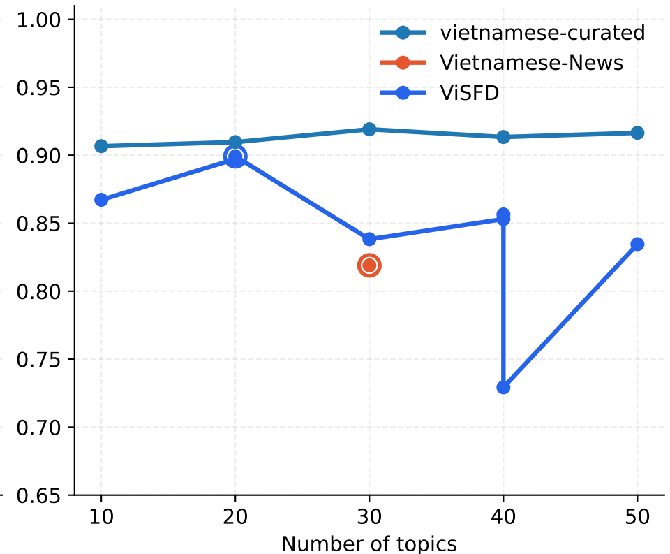
Aggregate interpretability
