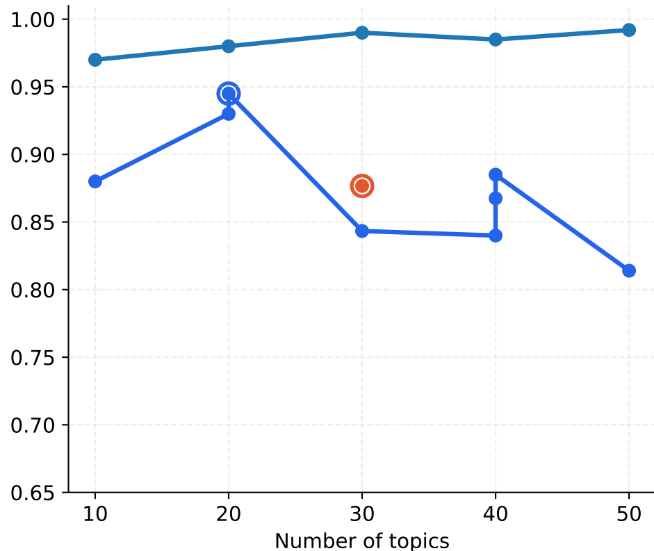
Topic diversity
