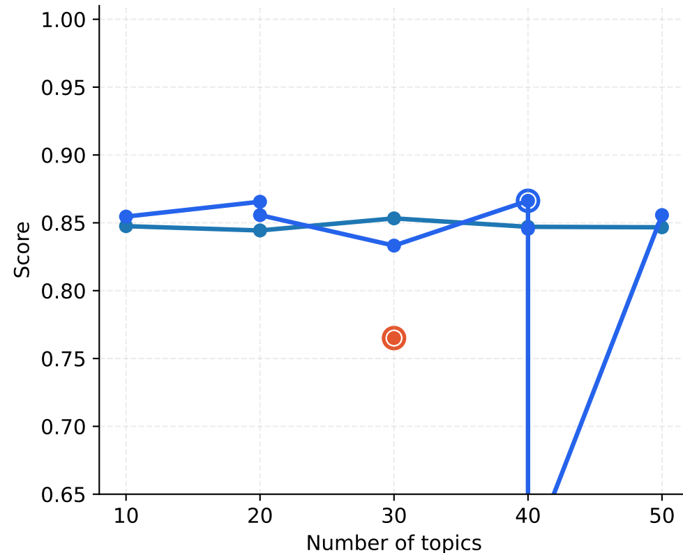
Embedding coherence
