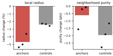
Figure 3: Fixed-encoder intervention test, one marker per seed. With the cycle-0 encoder frozen and every generated image inserted into the k NN index, the radius of the treated anchors falls about twice as far as that of matched controls, so the variants land in their own anchors’ neighborhoods. Purity falls about a third as much at the anchors.
