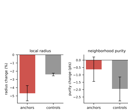
Figure 3: Fixed-encoder intervention test. With the cycle-0 encoder frozen and every generated image in the k NN index, the radius of the treated anchors falls about twice as far as that of matched unselected images, so the variants land in their own anchors’ neighborhoods, and purity falls about a third as much at the anchors. Bars are seed means with one standard deviation.
