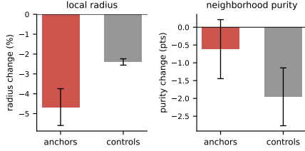
Figure 3: Fixed-encoder intervention test. With the cycle-0 encoder frozen and every generated image in the k NN index, the radius of the treated anchors falls about twice as far as that of matched unselected images, so the variants land in their own anchors’ neighborhoods, and purity falls about a third as much at the anchors. Bars are seed means with one standard deviation.
