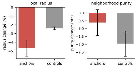
Figure 3: Fixed-encoder intervention test. With the cycle-0 encoder frozen and every generated image inserted into the k NN index, the radius of the treated anchors falls about twice as far as that of matched controls, so the variants land in their own anchors’ neighborhoods. Purity falls about a third as much at the anchors. Bars are the mean over seeds and the error bars are one standard deviation.
