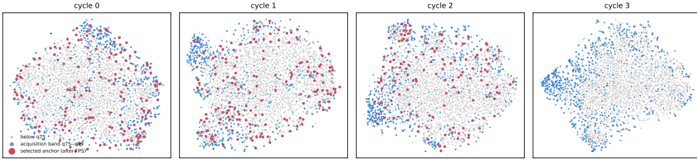
Figure 5: Where the acquisition budget is spent, projected to two dimensions with t-SNE, for one ImageNet-100-LT run. Grey marks scores below the 75th percentile, blue the q75–q99 acquisition band, and red the anchors farthest-point sampling selects from that band. The band occupies the periphery of the projection: over the panel shown, the rank correlation between k NN score and distance from the projection centre is +0.51, and band members sit at mean radius 34.6 against 25.5 for the rest. The anchors are spread across the band and not clustered inside it, which is the behaviour farthest-point sampling is included to produce. Each panel is projected separately because the encoder changes between cycles, so positions are comparable within a panel and not across panels. The panel contains original images only, so it shows which regions are targeted and not what the inserted samples do to them; Table 6 measures the latter directly.
