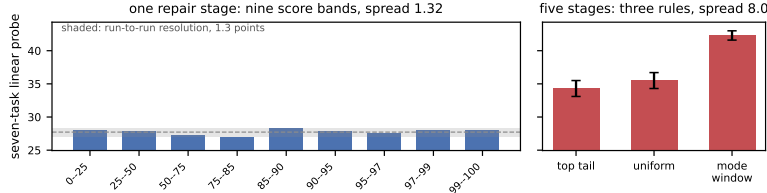
Figure 3: One repair stage against five. Left: nine bands of the k NN score distribution, each spending an identical budget after a single stage, all inside the shaded envelope, which is the run-to-run resolution of the pipeline measured by two rows of the robustness table that are provably the same experiment. Right: three acquisition rules under five stages at the same repair volume and optimizer budget. Rules indistinguishable after one intervention separate by 8.0 points once the signal is recomputed between them.
