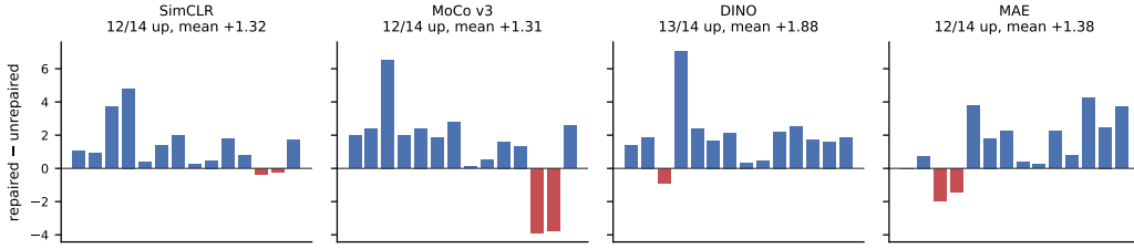
Figure 2: Repair against no repair for each of the four objectives, one bar per downstream measurement: linear probe and k NN on each of the seven datasets, from paired ViT-S runs at three seeds, both arms branching from one source checkpoint with the same number of post-branch updates. Appendix Tables 23 and 24 give the underlying accuracies. Blue is an improvement. The two losses under MoCo v3 are CIFAR-10 and CIFAR-100 under k NN.
