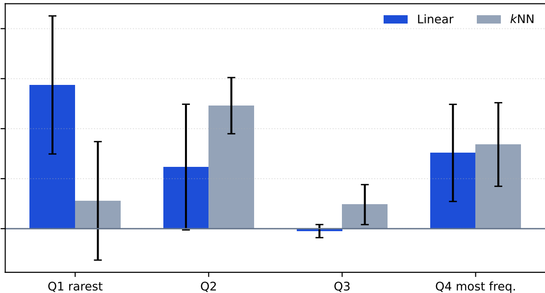
Lower-frequency classes benefit more on average under linear probing
