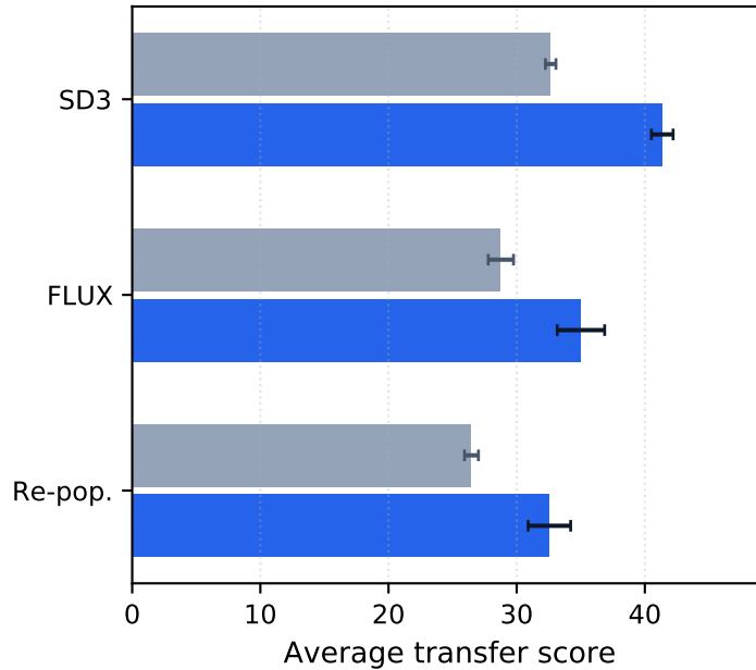
Generation
