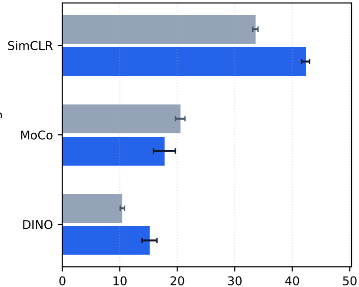
SSL objective
