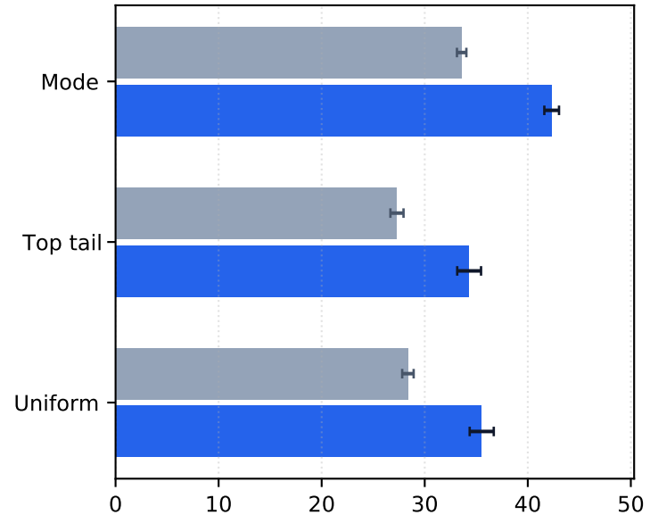
Selection
