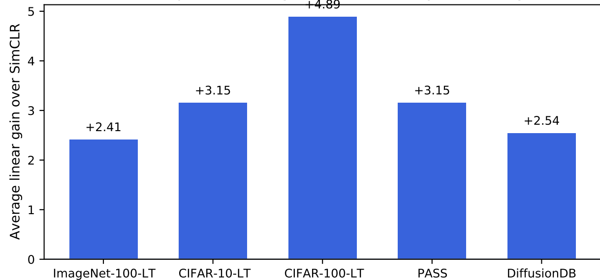
BRIDGE improves average transfer in every source regime
