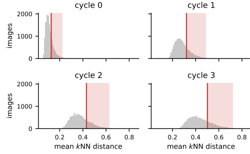
Figure 5: Score distribution over the four repair cycles of one ImageNet-100-LT run, with the 75th to 99th percentile band shaded and its modal bin marked, where the selector centers its pool. The distribution shifts to larger scores and broadens at every cycle, so the band is re-derived from the current representation instead of being fixed.
