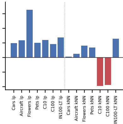
MoCo v3 12/14 up, mean +1.31
