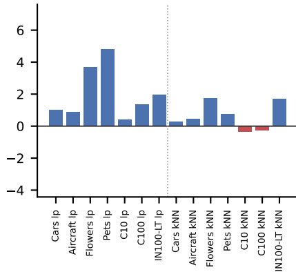
SimCLR 12/14 up, mean +1.32
