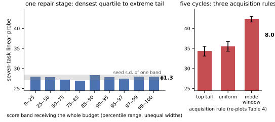
Figure 3: Left, nine bands of the score distribution of unequal percentile widths each receive the whole budget after a single stage, and their averages span 1.3 points (Appendix Table 22). The shaded region is one seed standard deviation of a single band’s seven-task mean, 0.66 points on average and between 0.35 and 0.93, so no pair of bands is separated at three seeds. Right, three acquisition rules under five cycles separate by 8.0 points, re-plotting the selection block of Table 4. Single-stage averages lie near 28 and five-cycle averages between 34 and 42.
