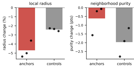
Figure 4: Fixed-encoder intervention test, one marker per seed. With the cycle-0 encoder frozen and every generated image inserted into the k NN index, the radius of the treated anchors falls about twice as far as that of matched controls, so the variants land in their own anchors’ neighborhoods. Purity falls about a third as much at the anchors.
