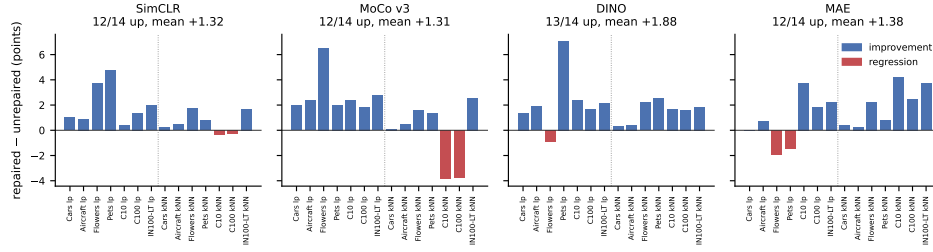
Figure 6: Repair against no repair for four objectives on ViT-S, one bar per downstream measurement (linear probe and k NN on each of seven datasets), from the paired runs of Table 3. Blue bars are improvements. Red bars are regressions, two for SimCLR and MoCo v3 (CIFAR-10 and CIFAR-100 under k NN), one for DINO (Flowers) and two for MAE (Flowers and Pets under the linear probe).
