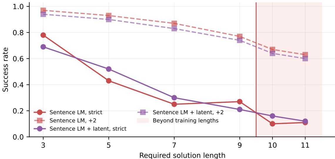
Longer problems expose an unresolved generalization gap (one seed)
