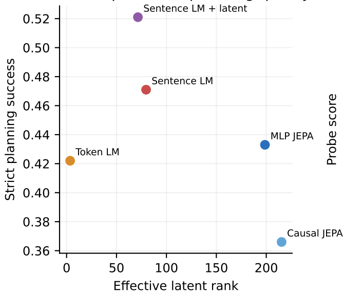
Non-collapse is not planning quality
