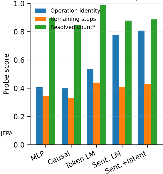
Different information is linearly accessible
