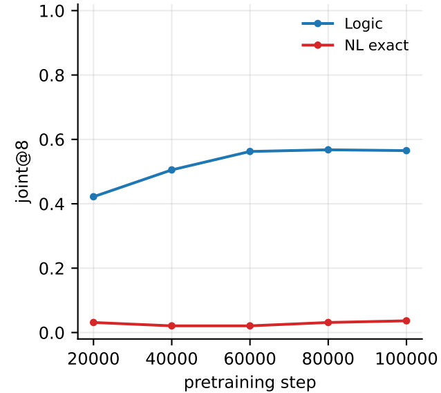
eval depth 1-10
