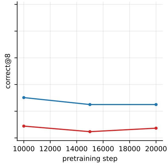
eval depth 12-20
