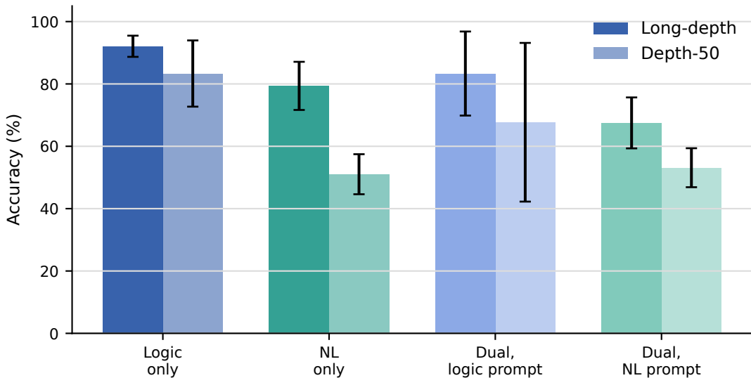
Conditioned dual training does not recover each single modality
