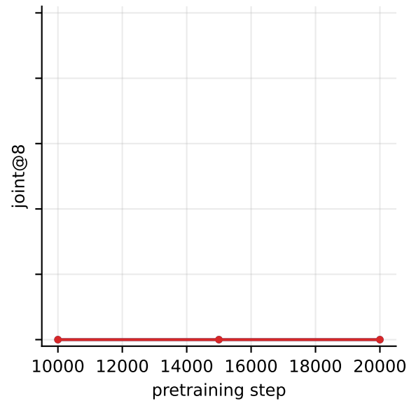
eval depth 12-20
