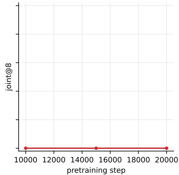
eval depth 25-30
