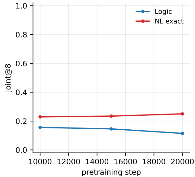
eval depth 1-10
