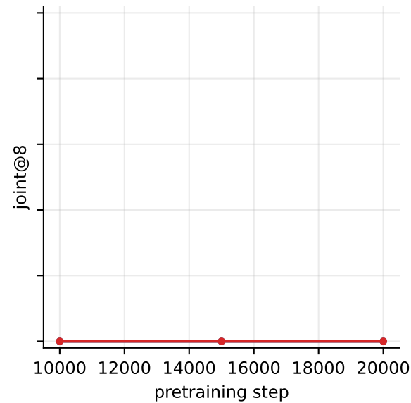
eval depth 40-50
