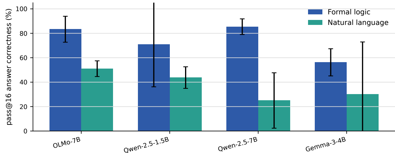
Depth-50 pass@16 across model families
