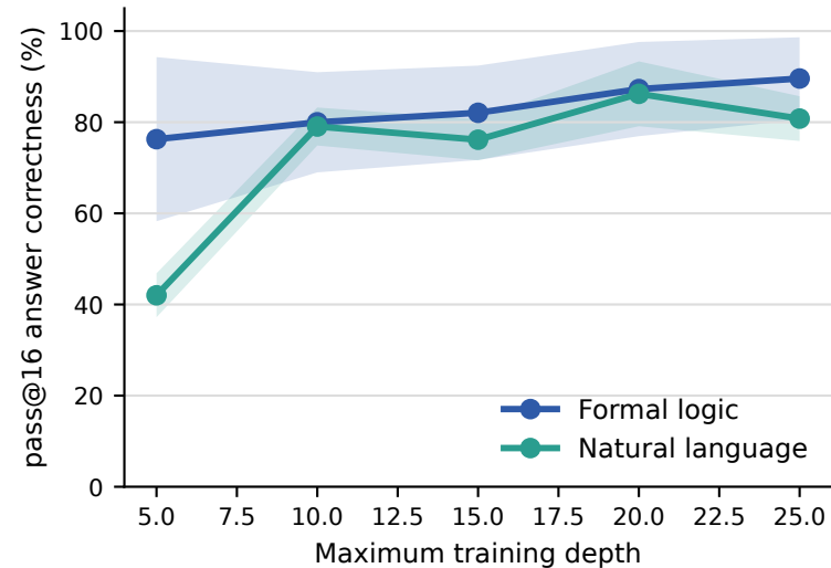
Hard-depth band pass@16
