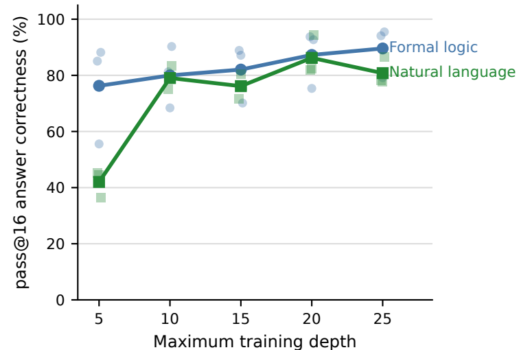
Constraint transfer is positive
