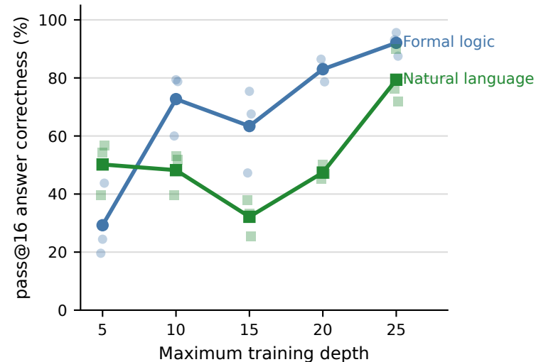
Formal traces extrapolate farther
