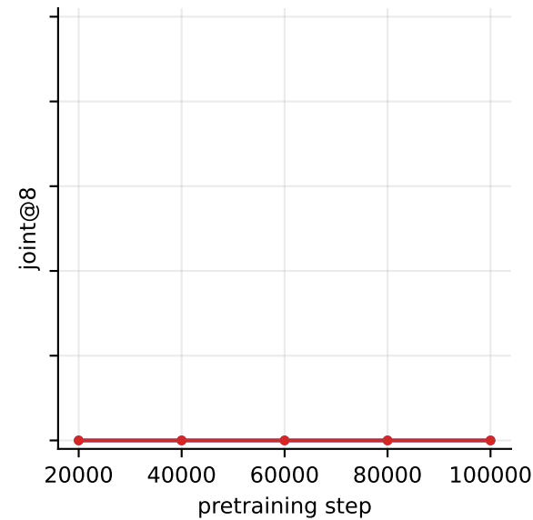
eval depth 40-50
