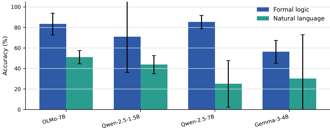
Depth 50 correctness across model families
