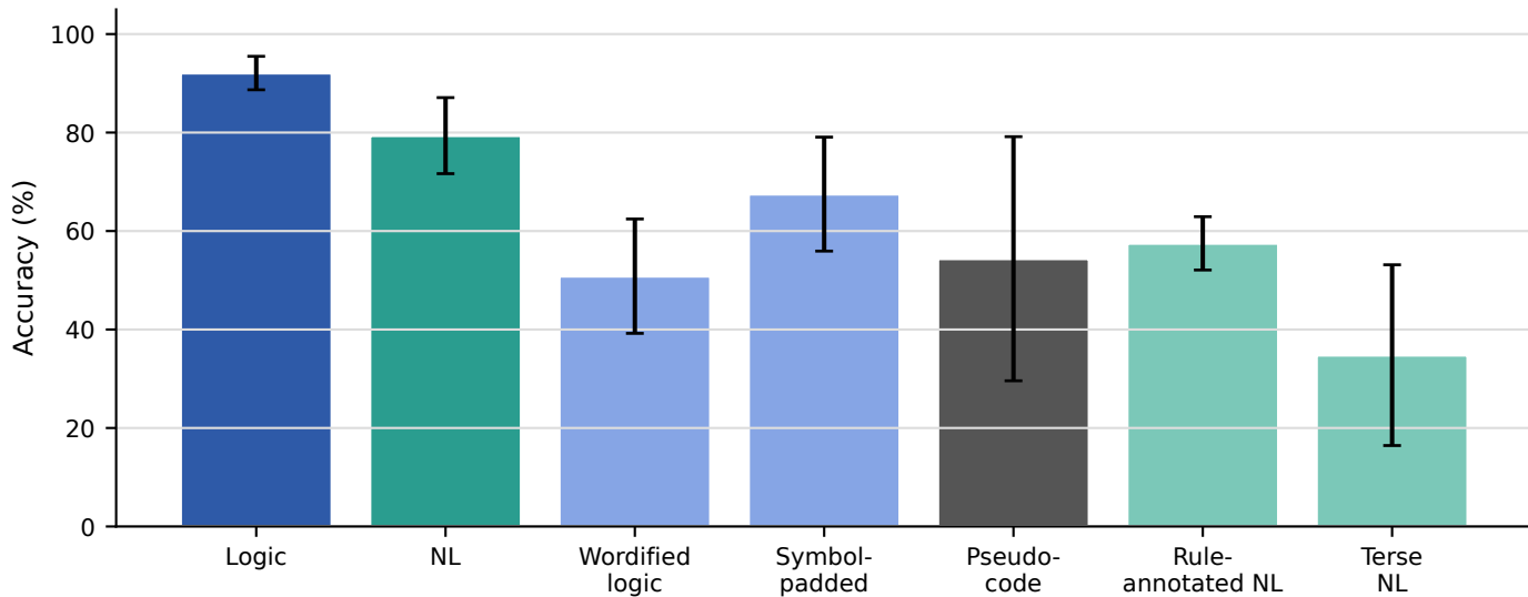
Surface syntax controls at maximum training depth
