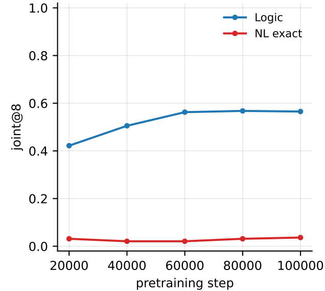
eval depth 1-10
