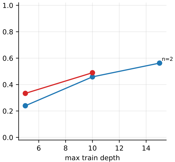
depth-50 correct@16
