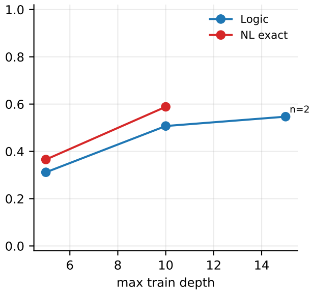
OOD correct@16
