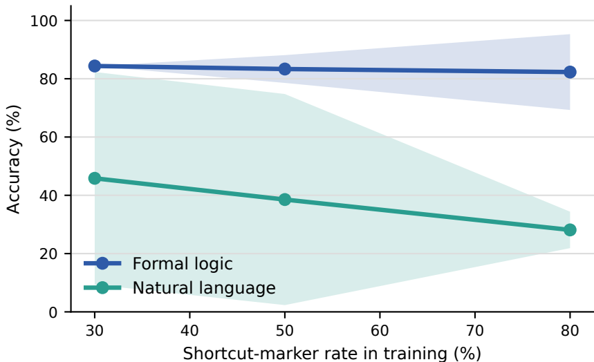
Depth 50 correctness under shortcut distractors
