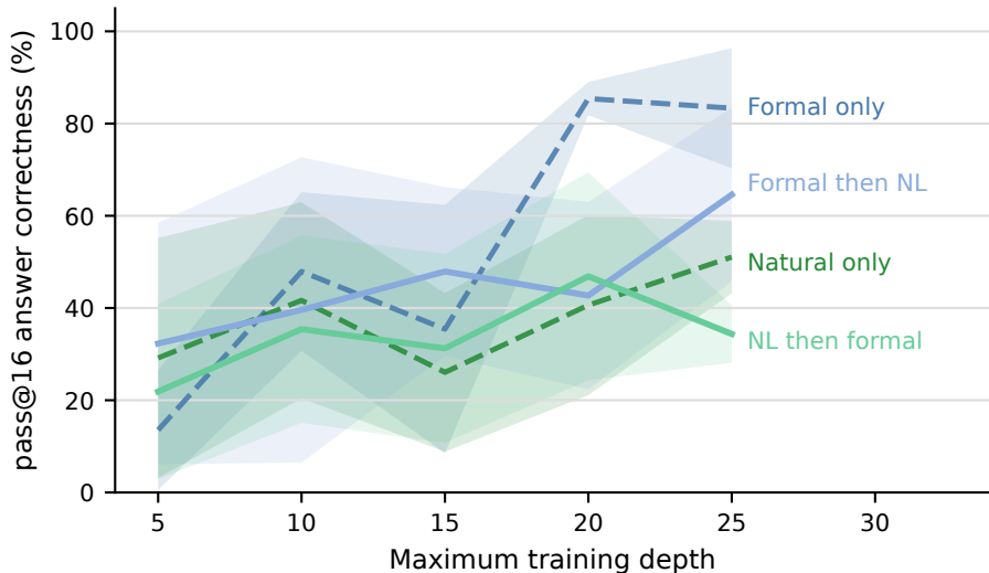
Hybrids trail formal-only extrapolation
