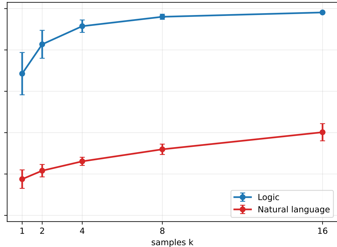
OOD correct and valid versus sample budget
