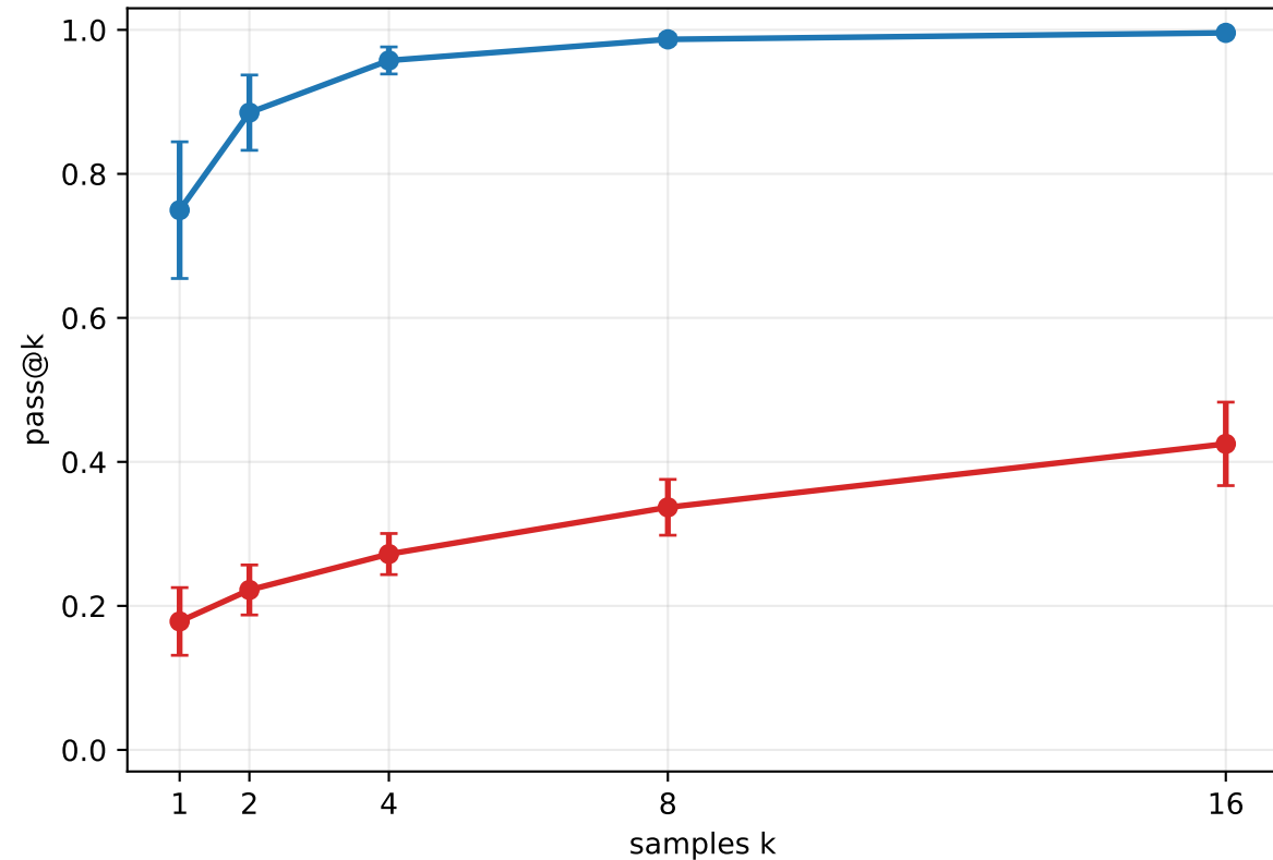
OOD correctness versus sample budget
