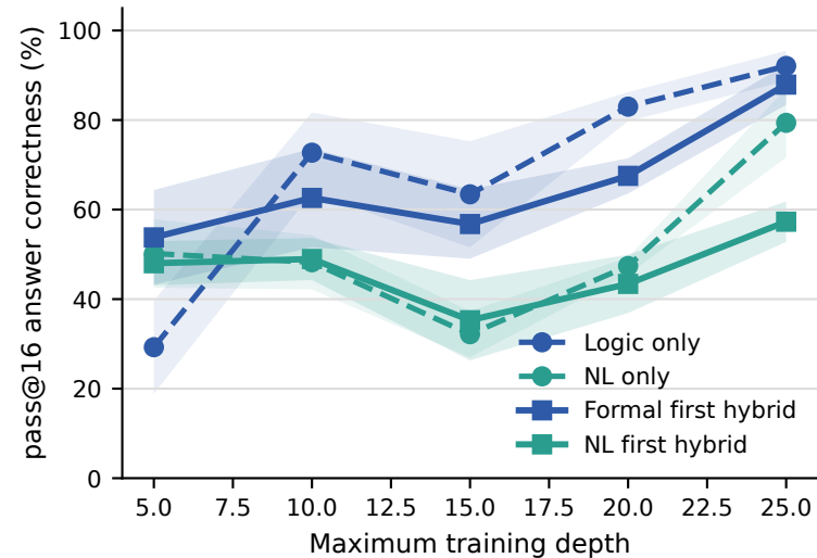
Long-depth band pass@16
