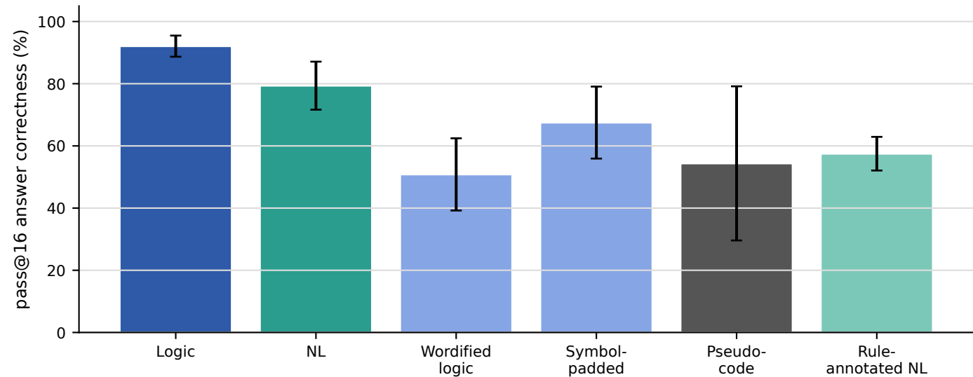
Long-depth pass@16 for syntax controls
