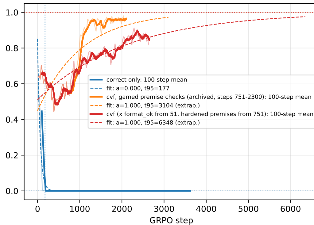
valid — Dolci prompts (math, wordprob, yesno)
