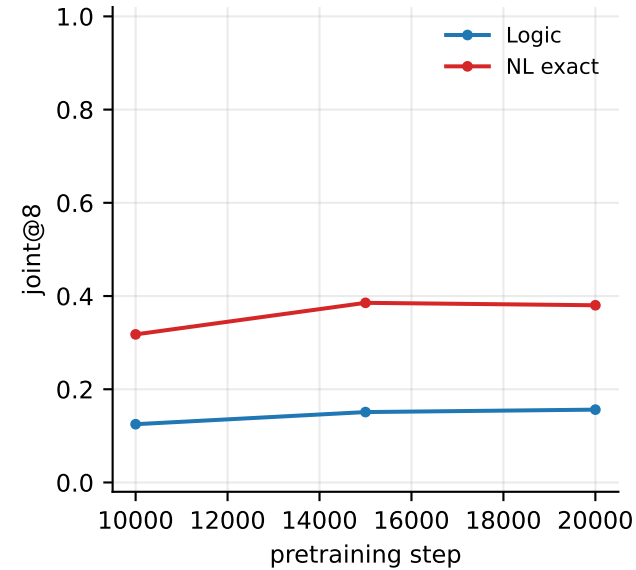
eval depth 1-10
