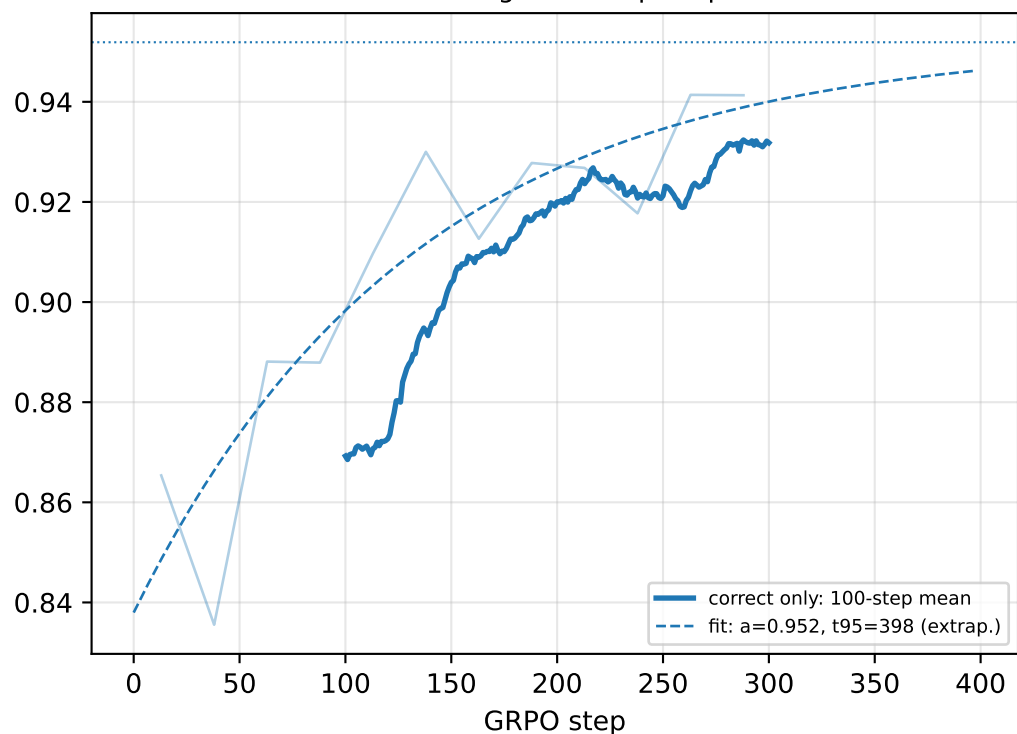
correct — Dolci prompts (math, wordprob, yesno)
