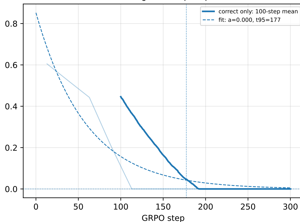
valid — Dolci prompts (math, wordprob, yesno)
