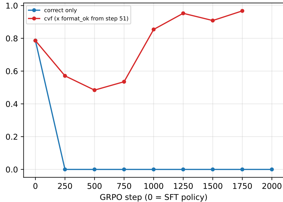
valid — Dolci gate, training benches (700 items)
