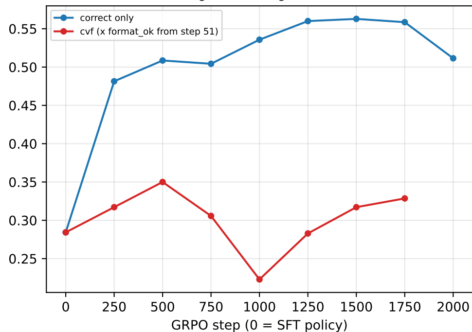
correct — Dolci gate, dapo + knowledge (250 items, OOD)
