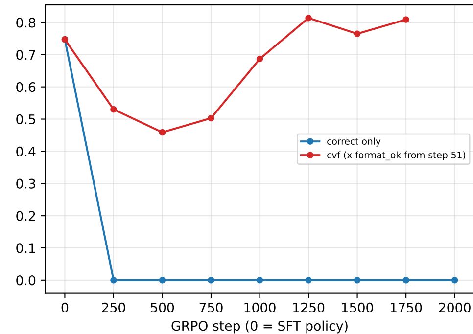
cvf — Dolci gate, training benches (700 items)
