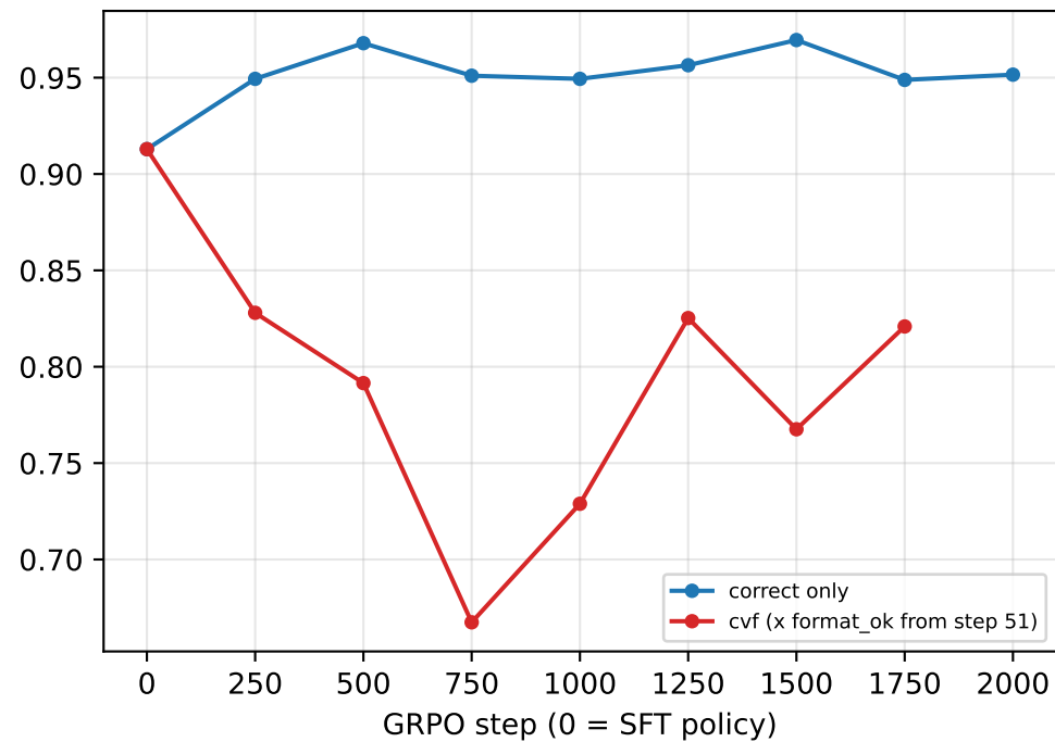
correct — Dolci gate, training benches (700 items)
