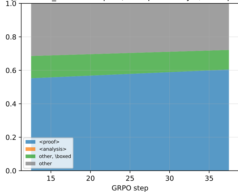
f (x format_ok from step 51): completion style, Dolci prompts
