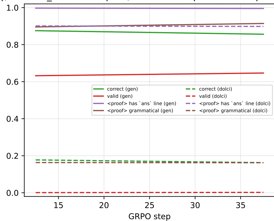
f (x format_ok from step 51): reward components and proof health
