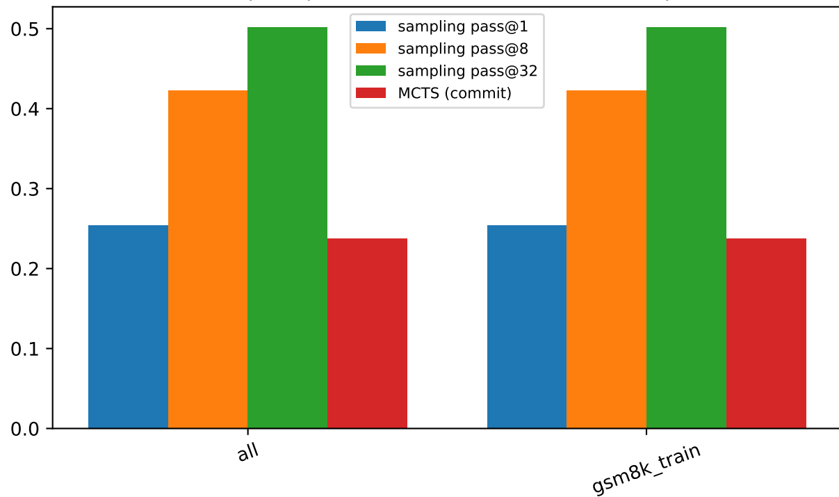
mixed prompts: share with a correct x valid proof
