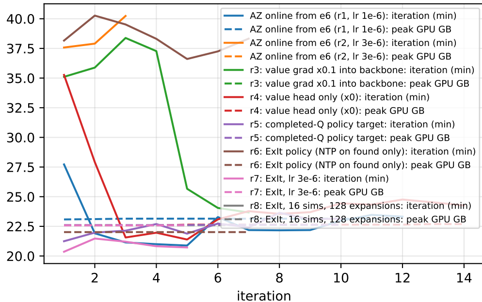
cost
