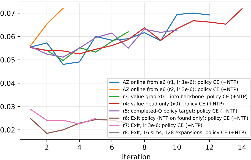
policy loss
