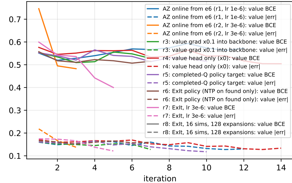
value loss
